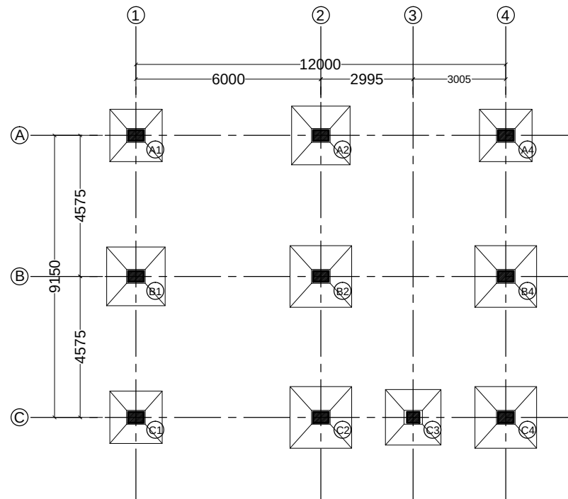
LAYOUT OF COLUMN & FOOTING
